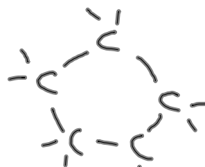
Cyclopentane
