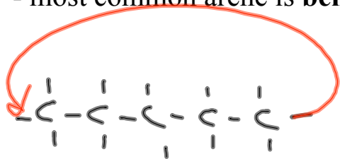
Pentane
