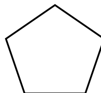
Cyclopentane
